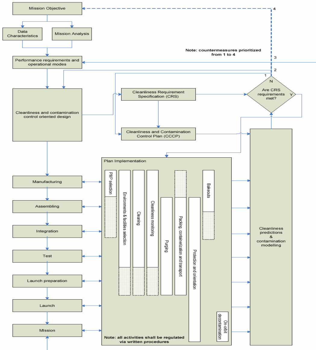
Figure 4-1 Cleanliness and contamination control process overview
